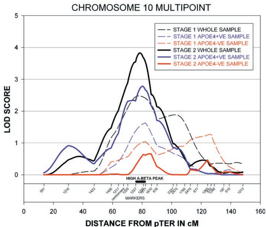
Fig. 1. Chromosome 10 multipoint map for LOAD. Multipoint linkage analyses were carried out with the program MAPMAKER/SIBS (11) on the whole sample (429 pairs), on pairs where both siblings had at least one APOE4 allele ( APOE4 +ve; 262 pairs), and on pairs where neither sibling had an APOE4 allele ( APOE4 -ve; 83 pairs). The region of linkage for high plasma A \beta 2 from the Ertekin-Taner et al. (13) report is also shown. Marker distances were taken from the Marshfield database (15).
