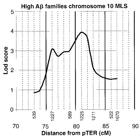
Fig. 1. Chromosome 10 multipoint plot. Robust multipoint lod scores on chromosome 10 were calculated for the five LOAD families that had an AD proband with extremely high plasma Aβ. The markers that were genotyped are shown below the plot. A maximum MLS of 3.93 is at 81 cM between D10S1227 and D10S1211.
